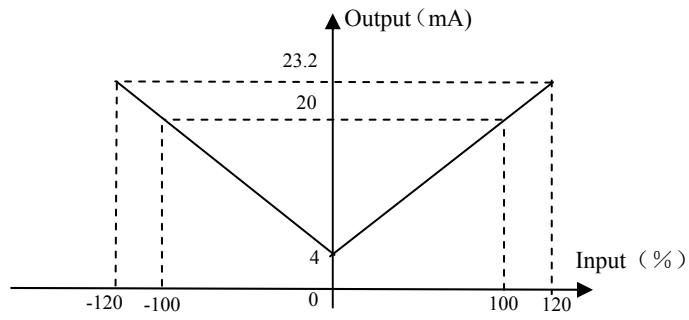
4mA~20mA Input-Output characteristic curve
